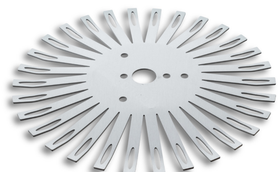
Biegeform F bend form F
